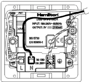
Wiring 13Amp Switched Single Sockets with USB Charging Outlet — Neutral — Earth — Live
