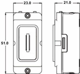
Hamilton® GRID-IT GK21 20AX 2 Way Key Switch Module
