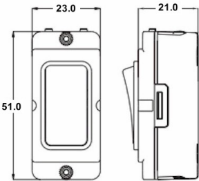
Hamilton GRID-IT GR21 10AX 2 Way Rocker Module
